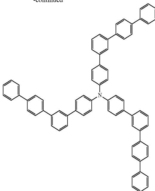
Objective compound 3
