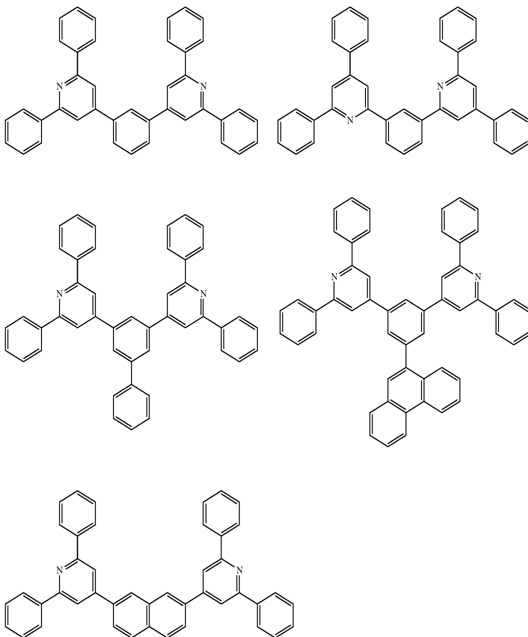
[Chem 8]
